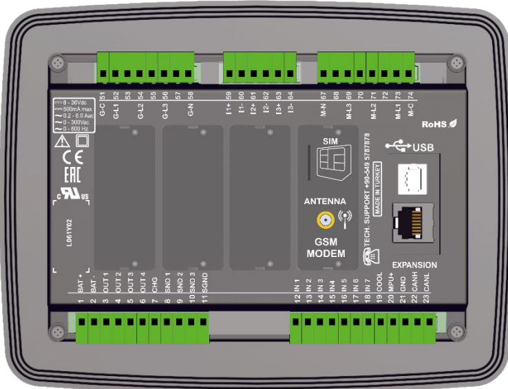
Backpanel view
